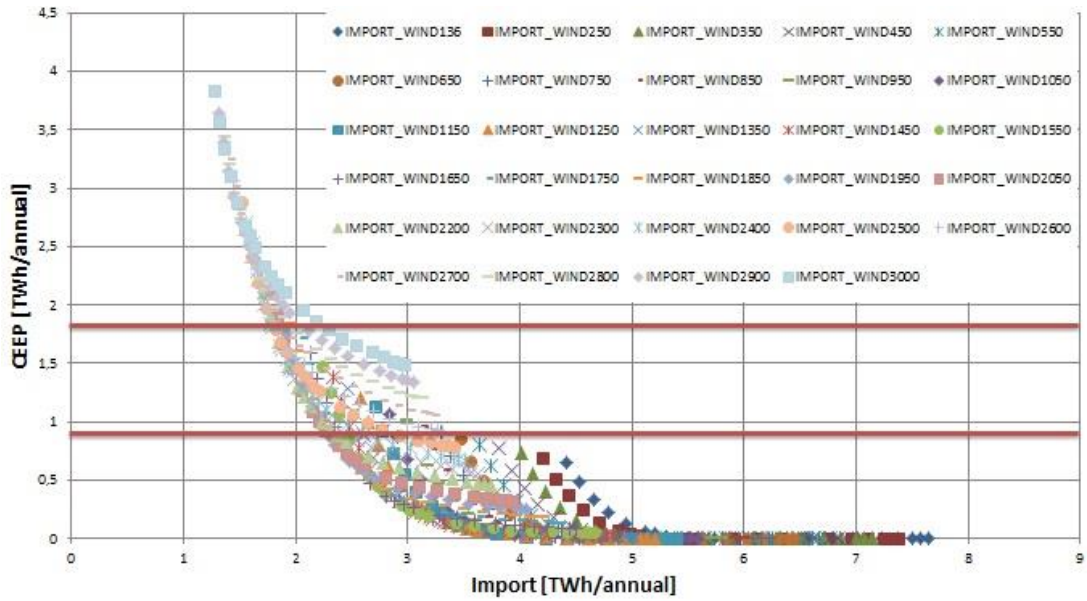
Figure 12. CEEP-Import chart with constant wind capacity
