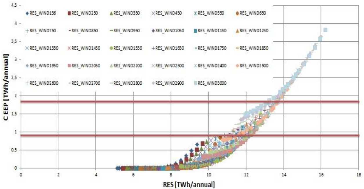
Figure 10. CEEP-RES chart with constant wind capacity
