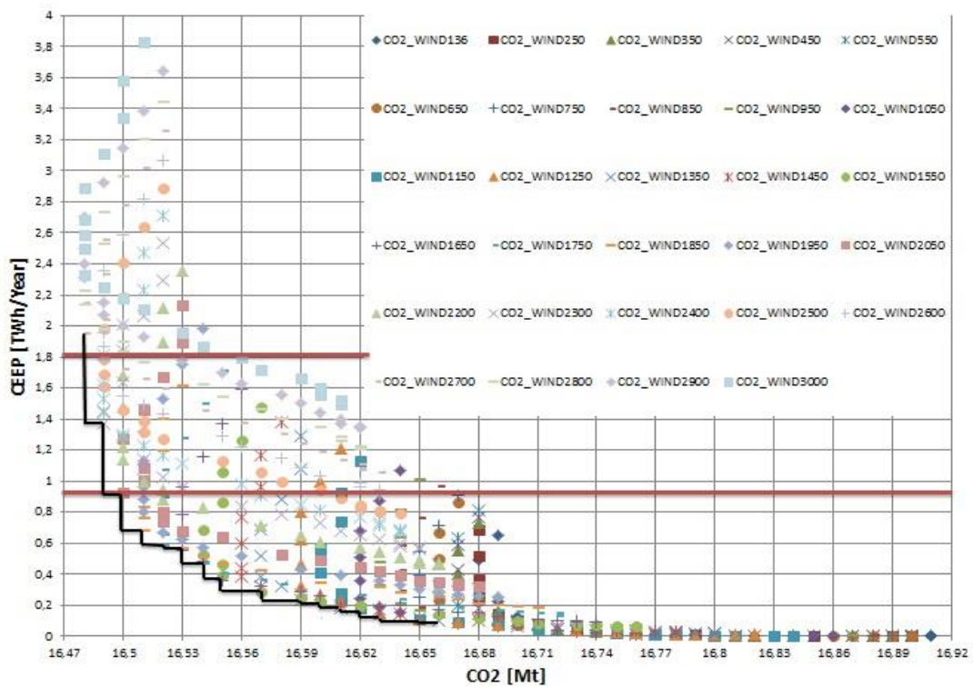
Figure 6. Pareto analysis of scenarios in case when the wind is base technology
