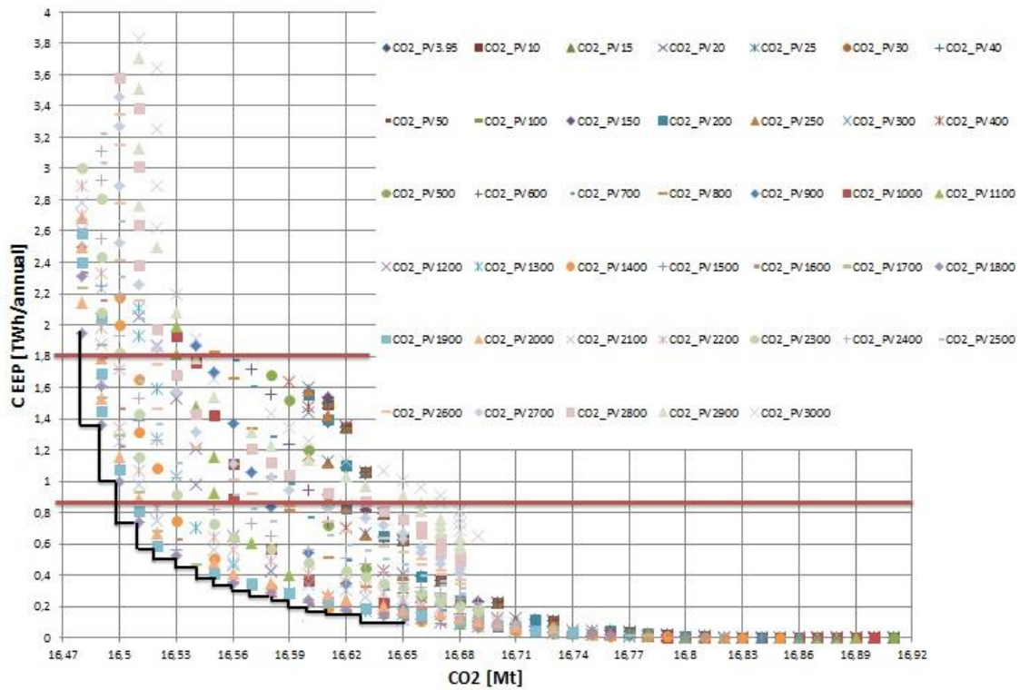
Figure 5. Pareto analysis of scenarios in case when PV is base technology
