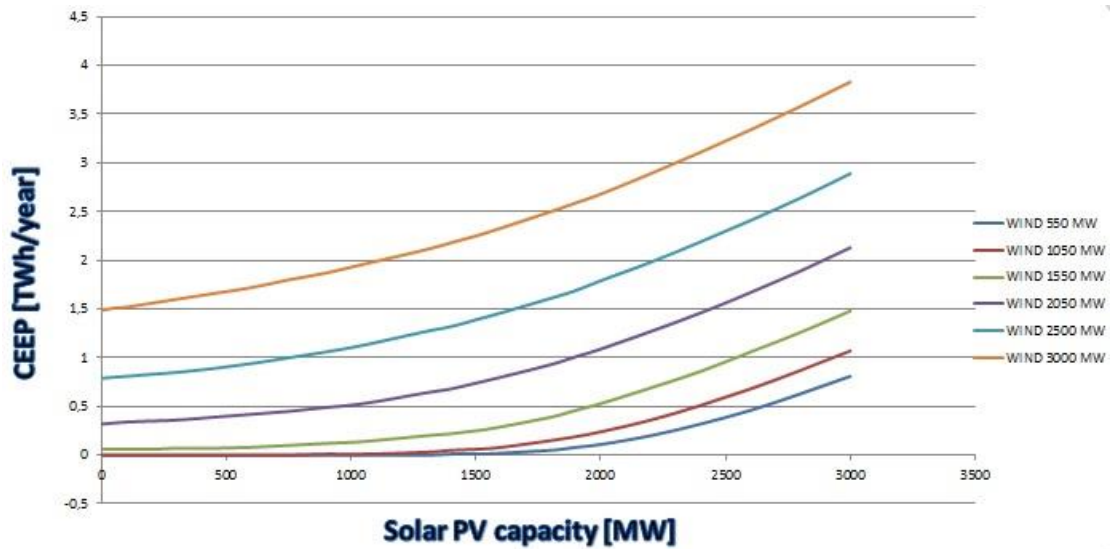
Figure 4. Growth of CEEP with increase in installed PV capacity
