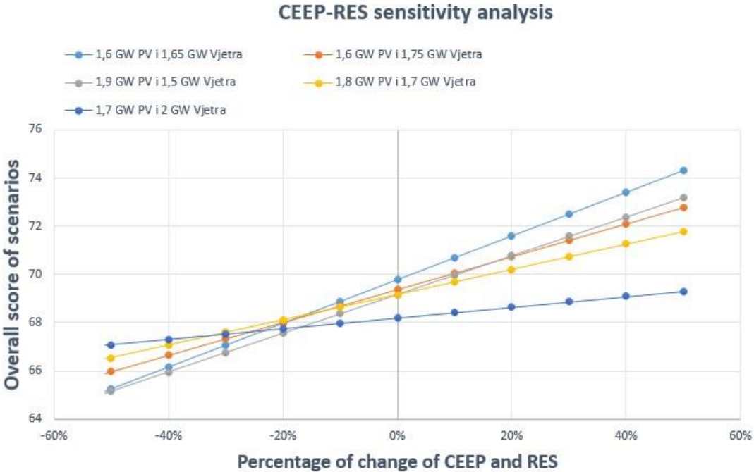
Fig 13. CEEP-RES chart for a change in the weight factor
