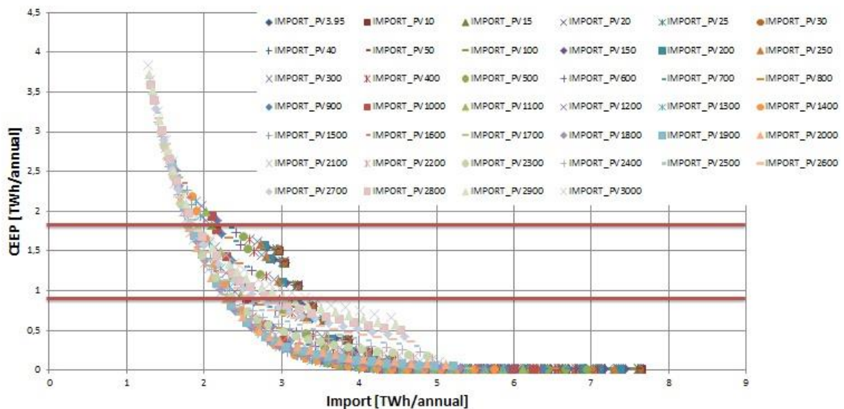
Figure 11. CEEP-Import chart with constant PV capacity
