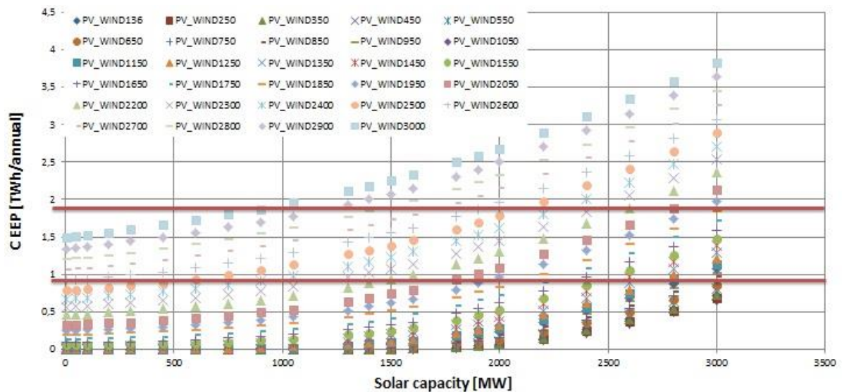
Figure 8. CEEP-Solar PV capacity chart
