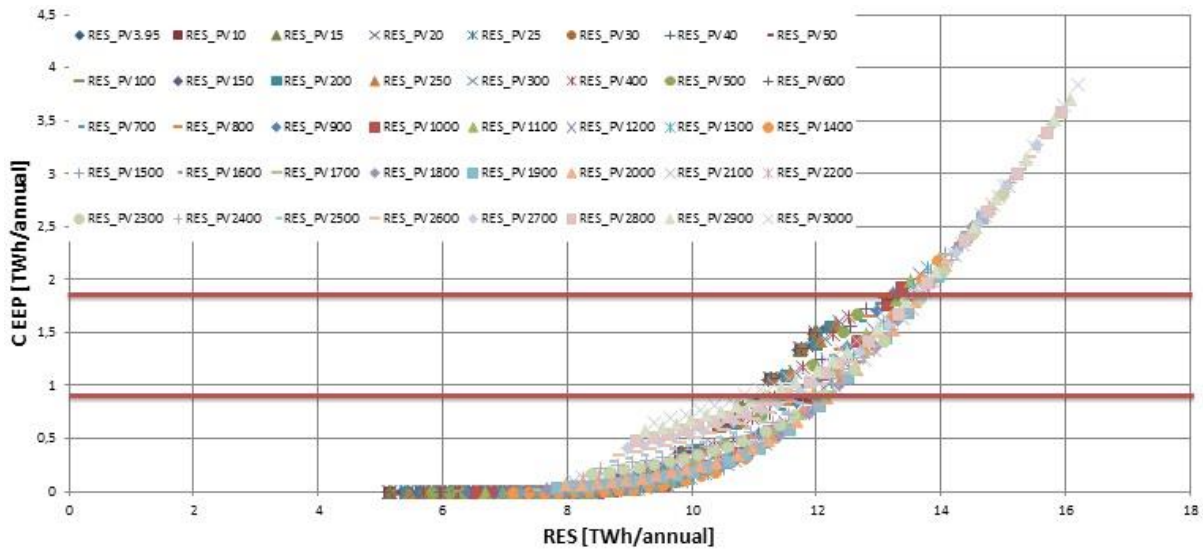
Figure 9. CEEP-RES chart with constant PV capacity
