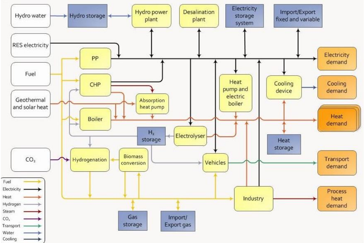
Figure 1. Schematic model of the EnergyPLAN tool
