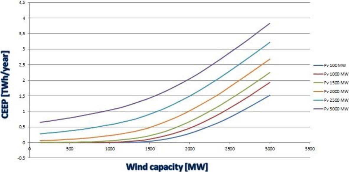
Figure 3. Growth of CEEP with increase in installed wind capacity
